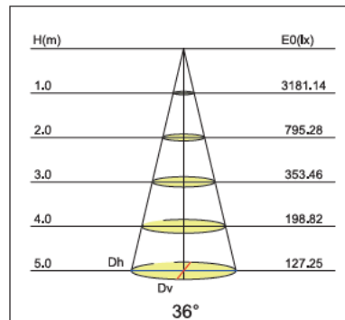
Typical light distribution for 25W4000K 36°
