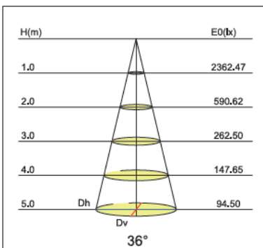
Typical light distribution for 19W4000K 36°
