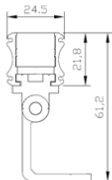
Angle Adjustable Bracket
